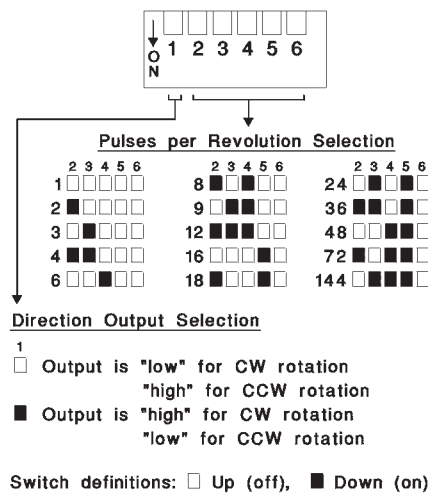
Figure 1 - Configuration Switches
